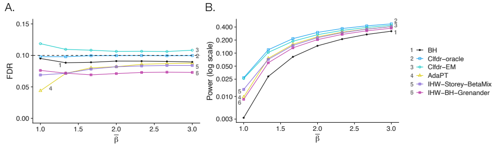
Figure 4: Simulation for multiple testing with a continuous covariate: A. False discovery rate in model (14) for six methods. The x -axis corresponds to a simulation parameter that is monotonically related to the strength of the signal for the alternatives. B. Power in model (14) for the same six methods. The nominal \alpha is equal to 0.1 throughout and results are averaged over 400 Monte Carlo replicates.
