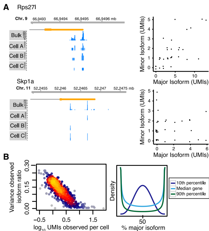
Figure 4. Raw isoform count data is noisy.
