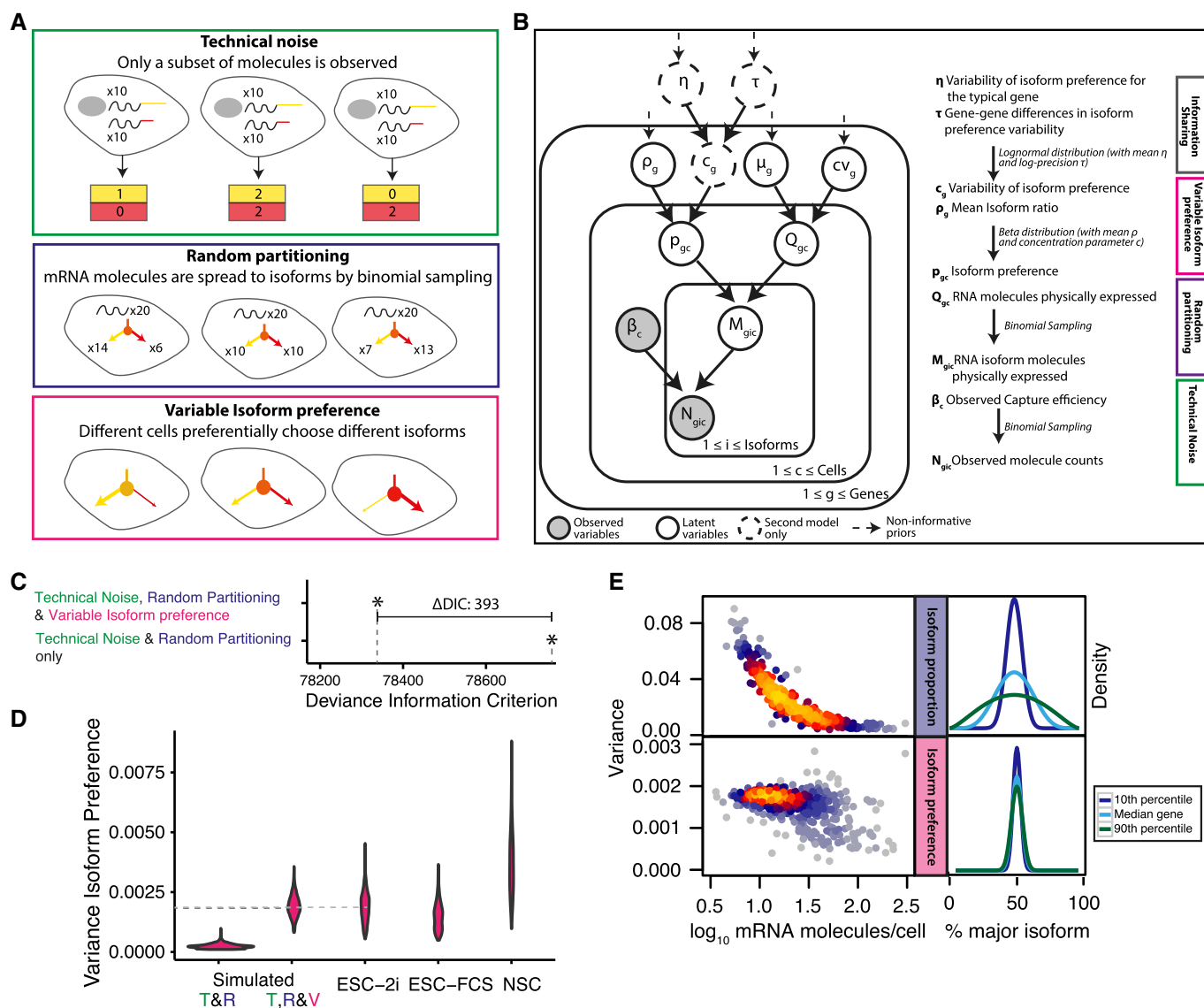
Figure 5. Isoform preference is different in different cells.
