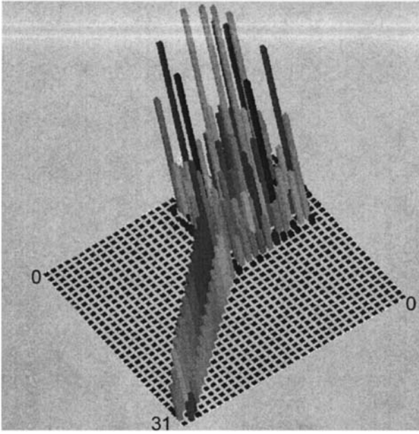
FIG. 2. Representation of the (N \times N) -matrix \mathbf{w}_{kj} formed by the various rates for the transition between the Floquet states for the Hamiltonian (10). The matrix element \mathbf{w}_{00} is found in the upper corner. The parameters are \alpha = 20 , \beta = 0.418 , \hat{T} = 4.5 , N = 32 , and m_{\max} = 2048 .
