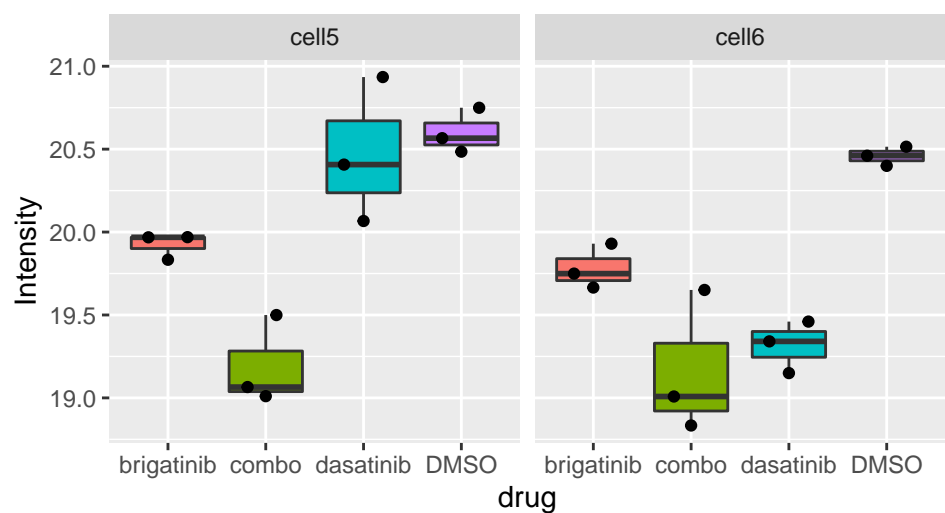
Plekha6_S973
