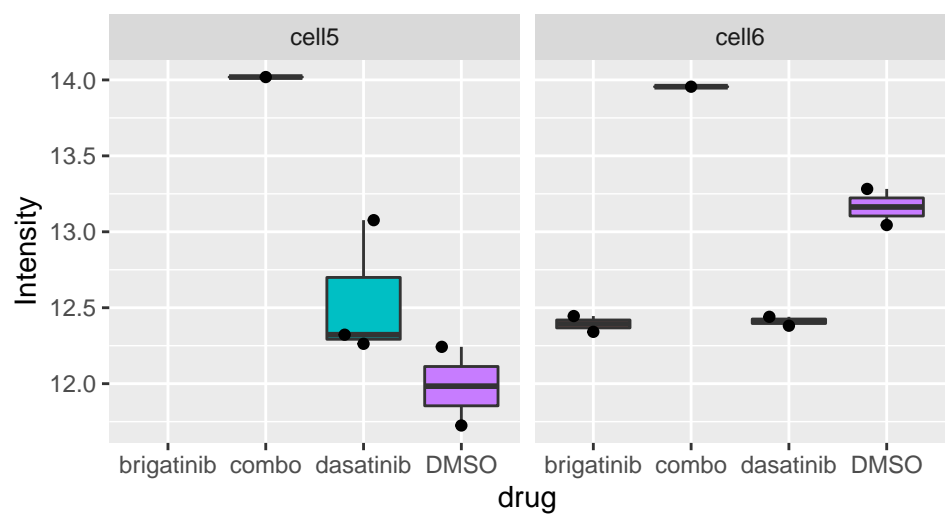
Lsm11_S15
