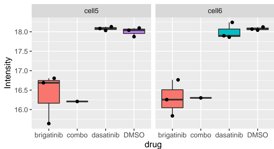
Mybbp1a_T1277
