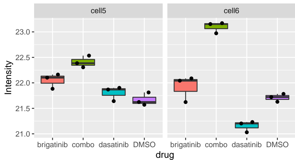
Srm2_S1876
