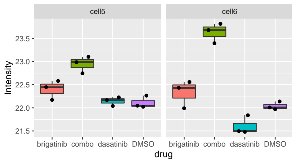
Srm2_S1912
