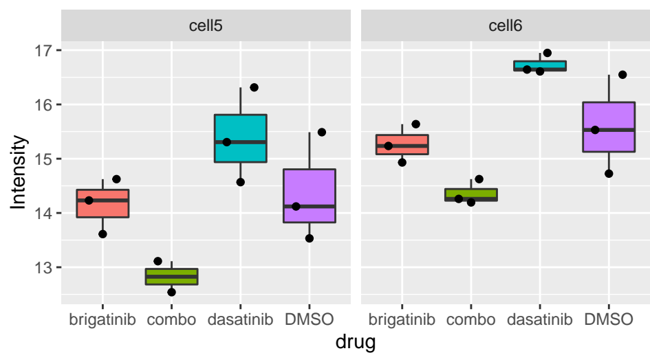
Xpc_S875
