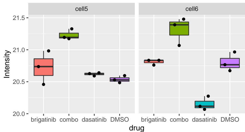
Pcyt1a_S319
