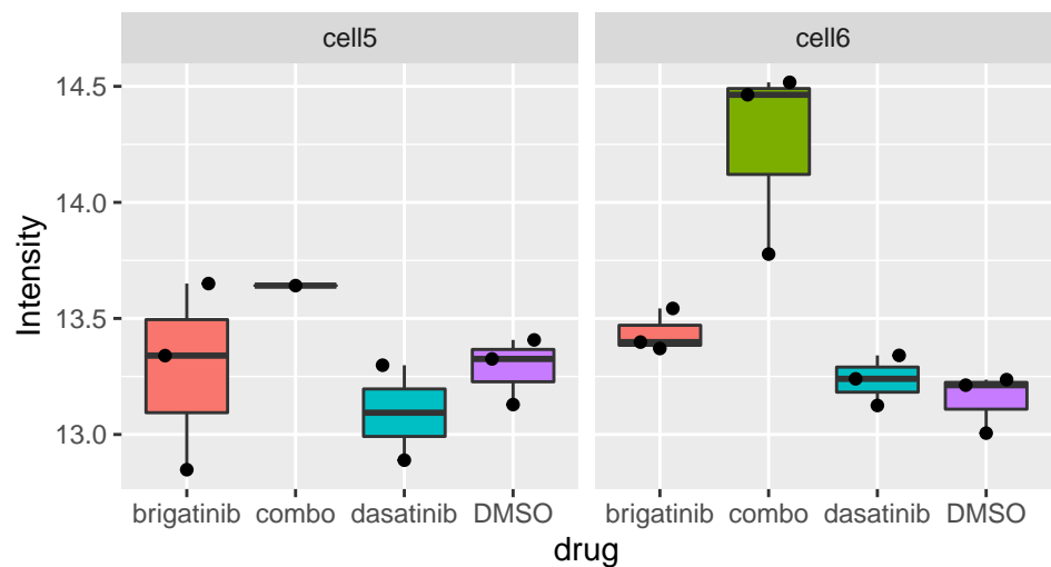
Top2b_S1539
