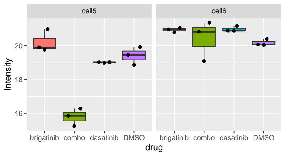
Map1b_S2207
