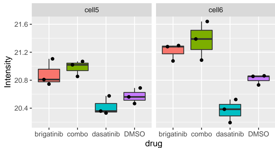
Mybbp1a_T1190
