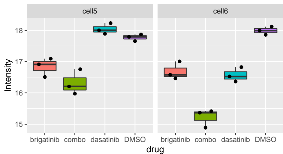
Camsap1_S553
