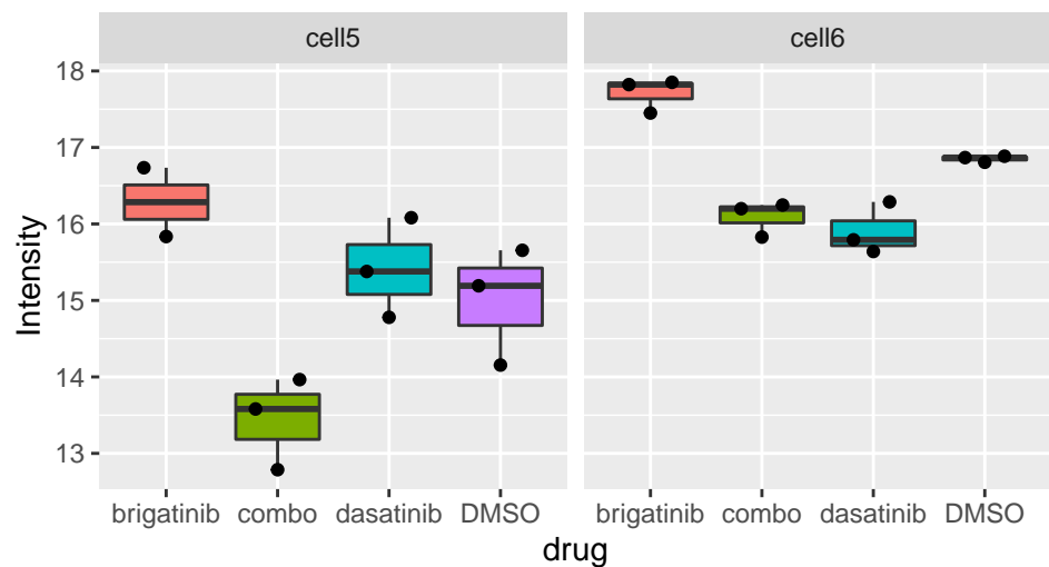
Smc1a_S957
