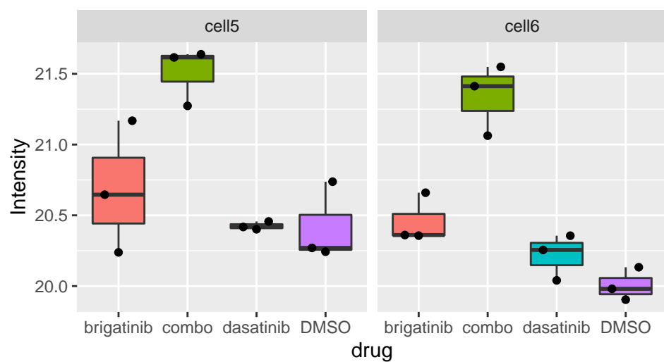
Srsf1_S199
