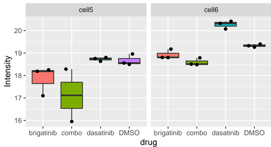
Wdr44_S405
