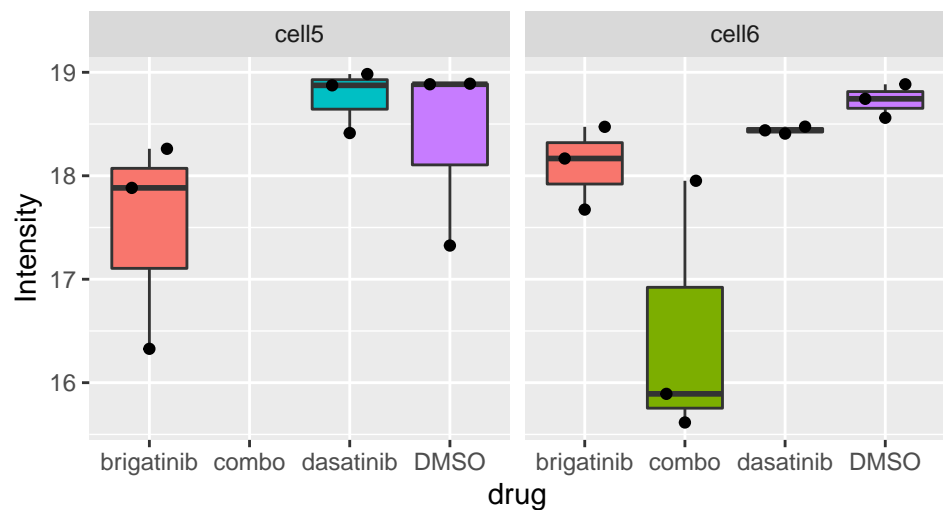
Plekhg3_S737
