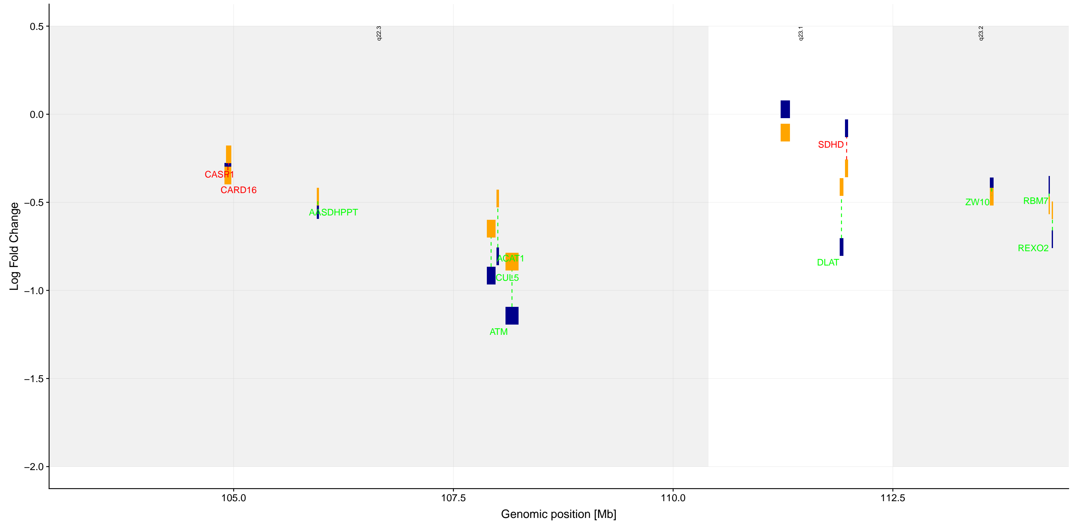
Log fold change comparison(11q)
