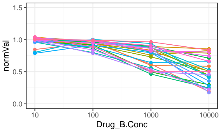
OT-82
