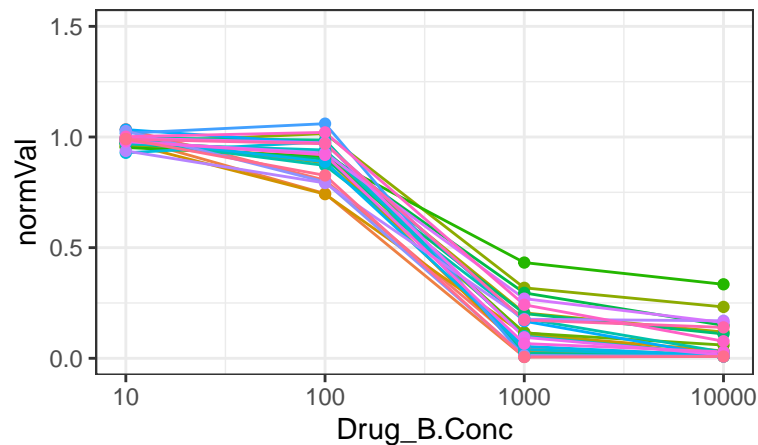
FCCP
