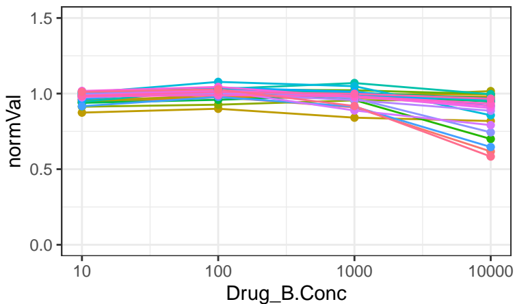
CAY10566
