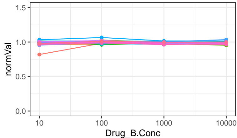
Gamitrinib
