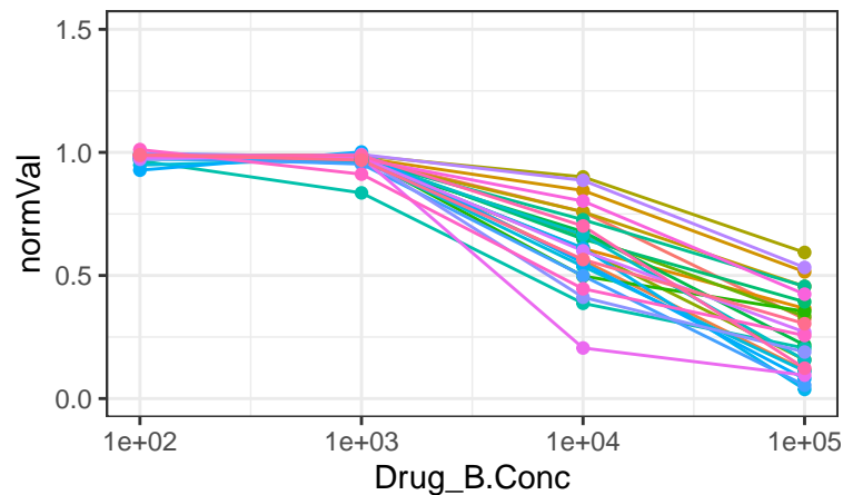
C75
