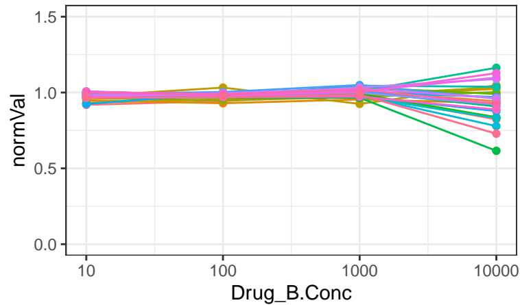
MK886
