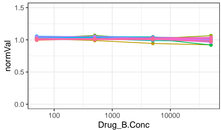
Hydroxychloroquine Sulfate
