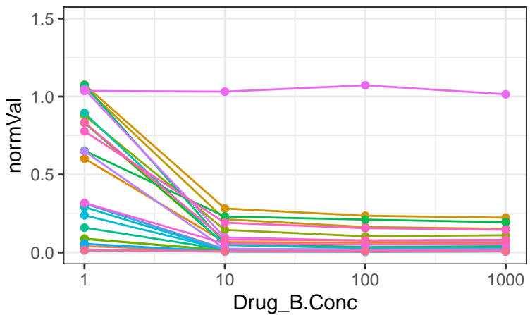
OT-82
