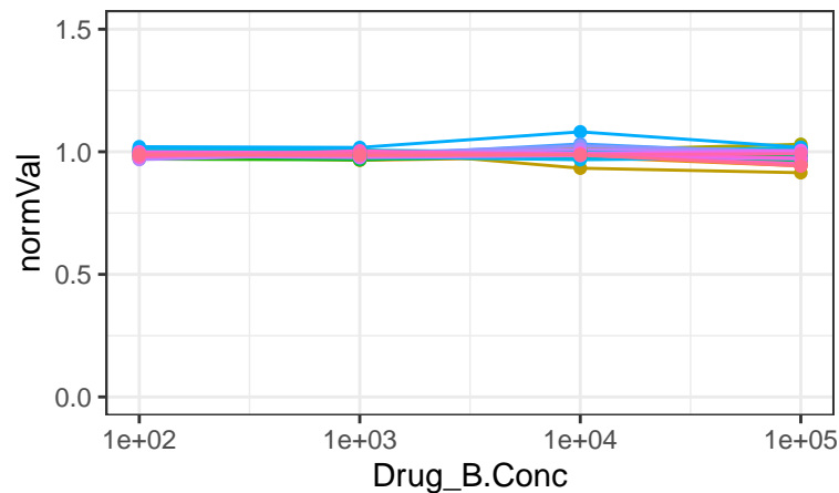
Lonidamine
