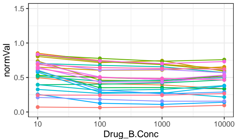
IACS-010759
