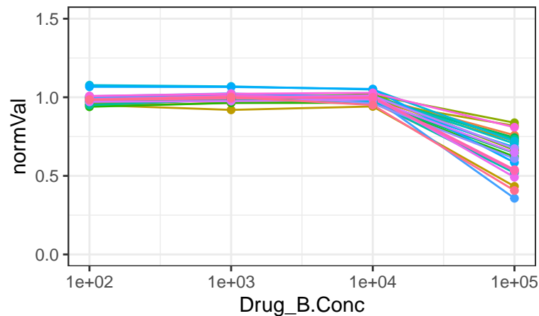
BAY-876
