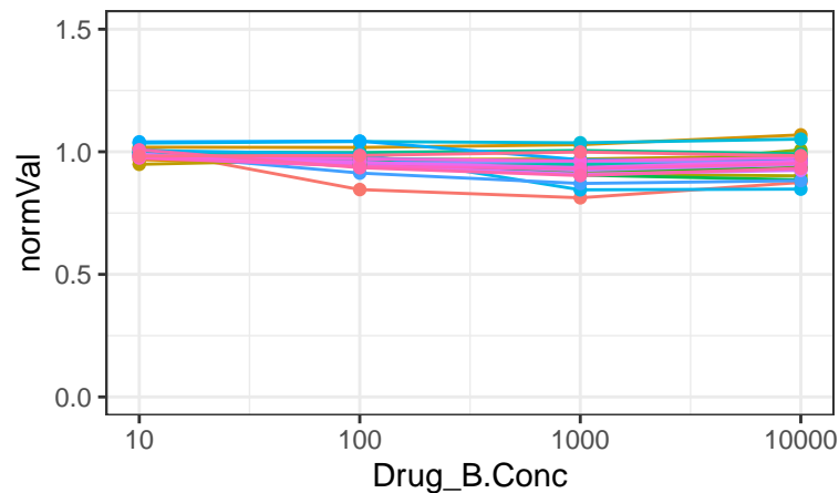
ND-646
