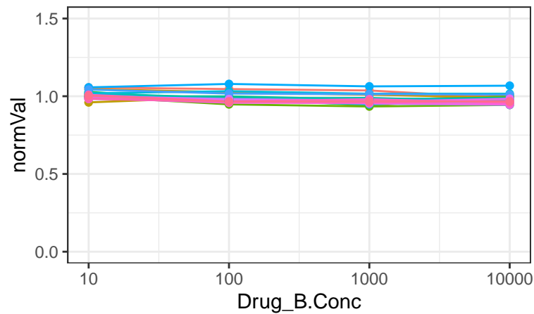
Lonidamine
