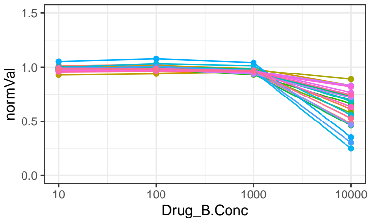
Dorsomorphin
