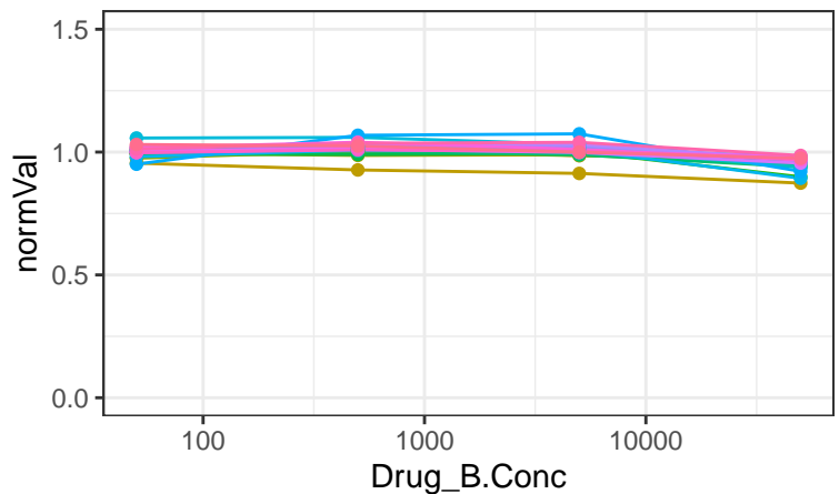
C2 ceramide
