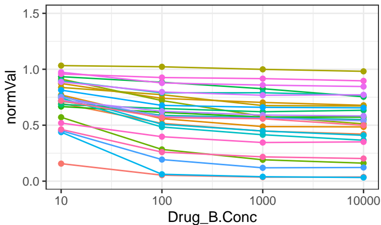
IACS-010759
