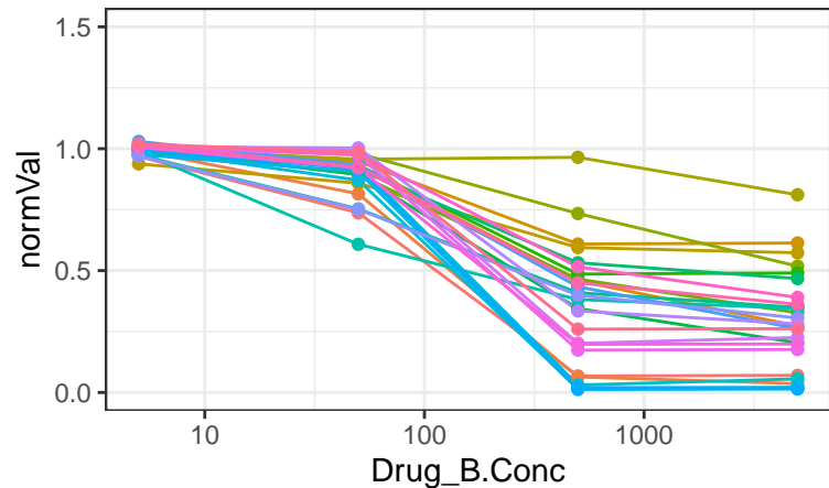
Compound 3K
