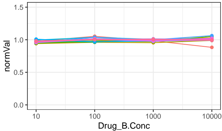
MK2206
