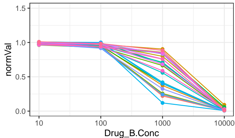
C646
