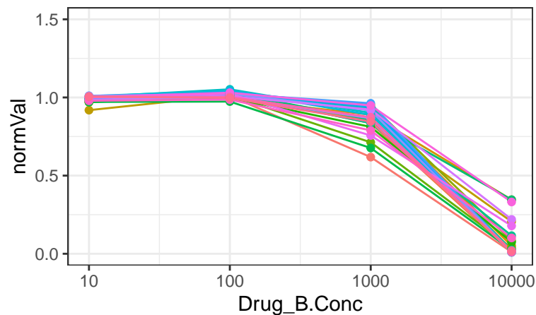
FCCP
