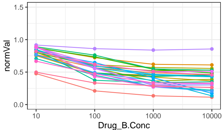
2-DG
