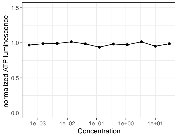
JNJ-28312141
