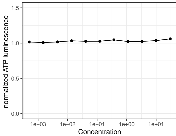
Rapamycin
