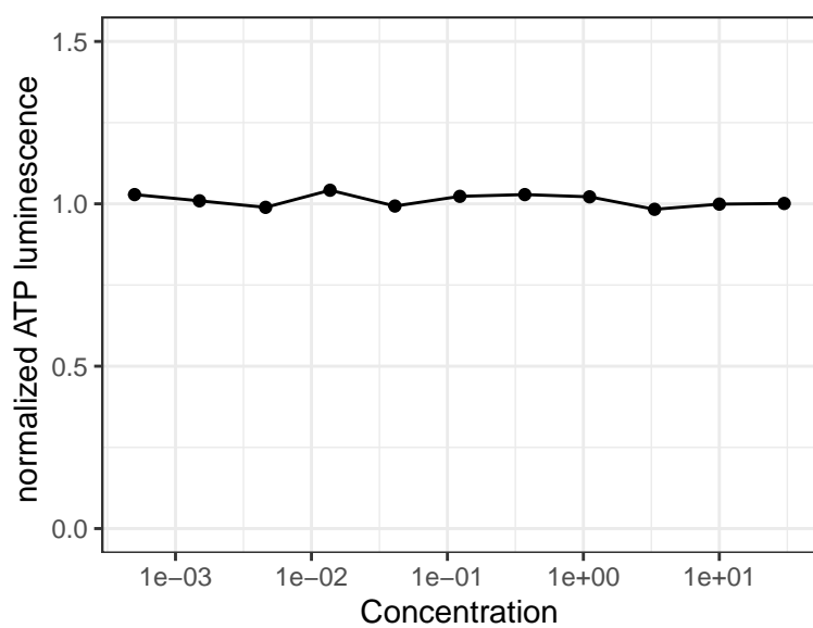
VO-Ohpic
