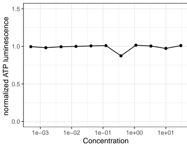
BX-795
