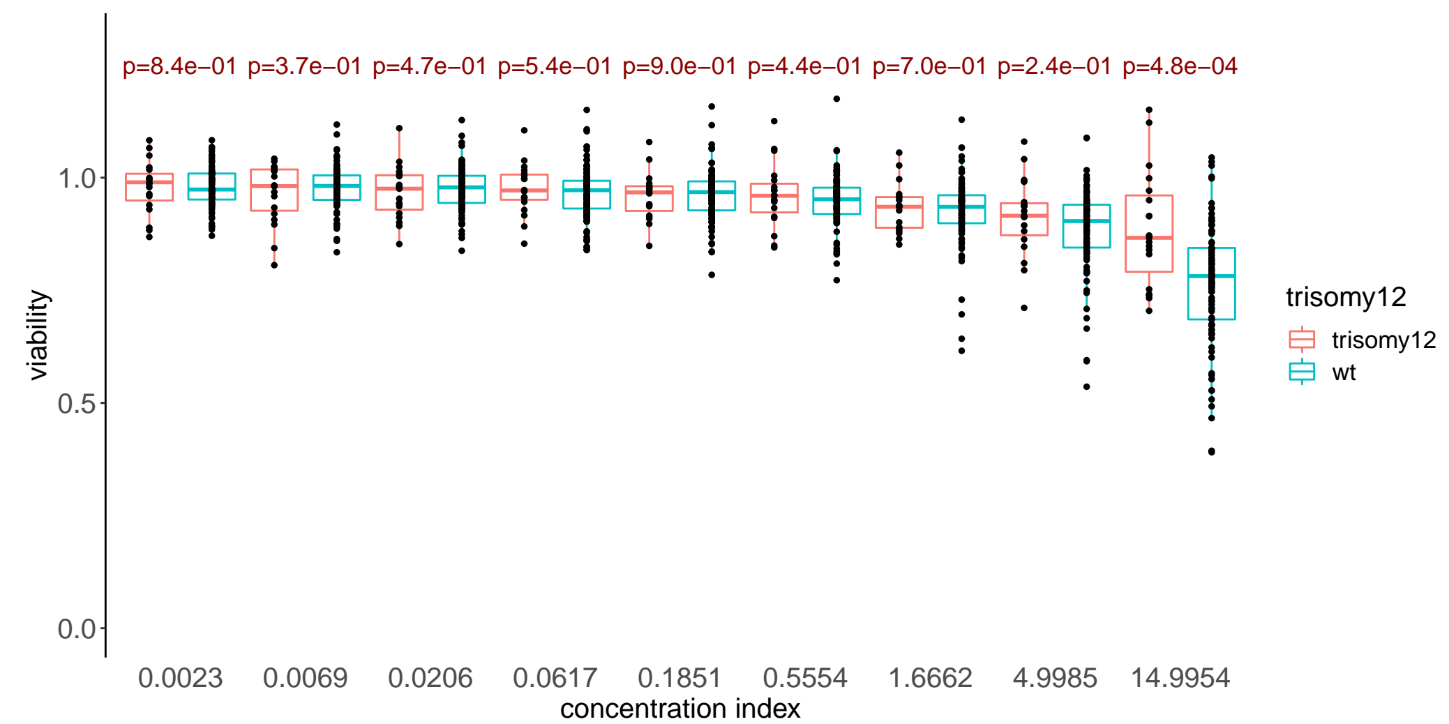
LGK-974
