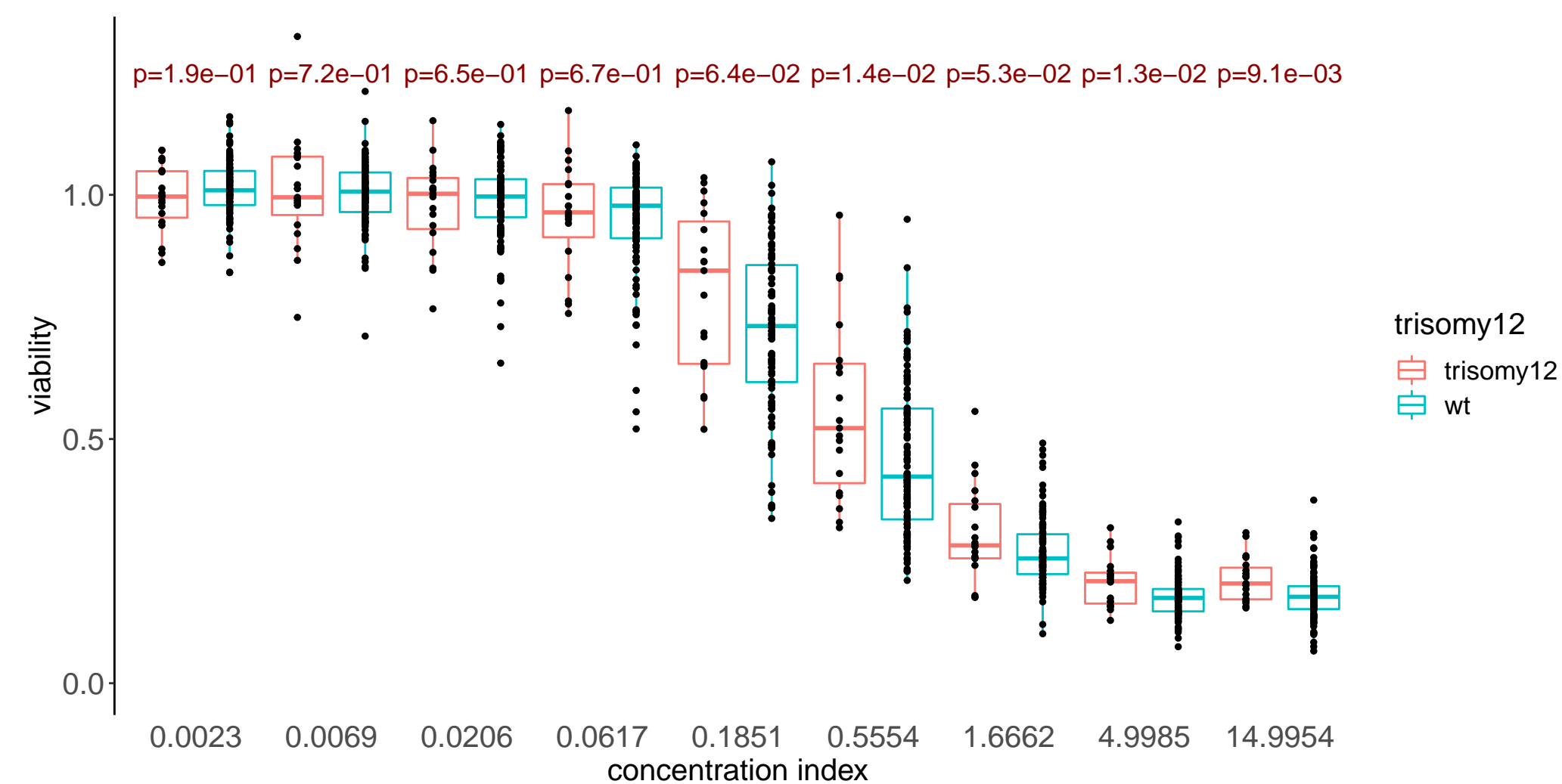
AT7519
