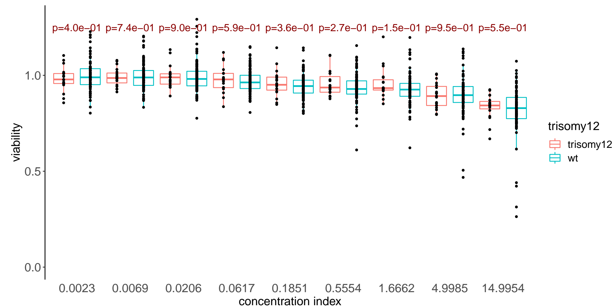
TCS PIM-1 1
