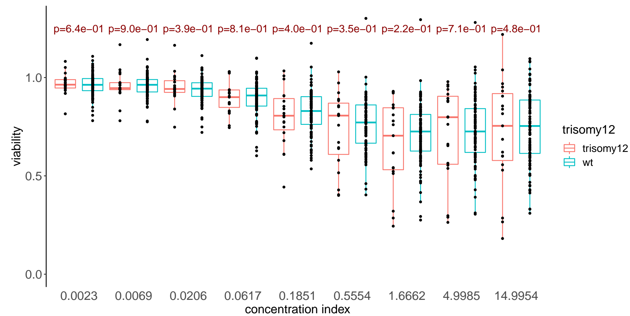
Pictilisib
