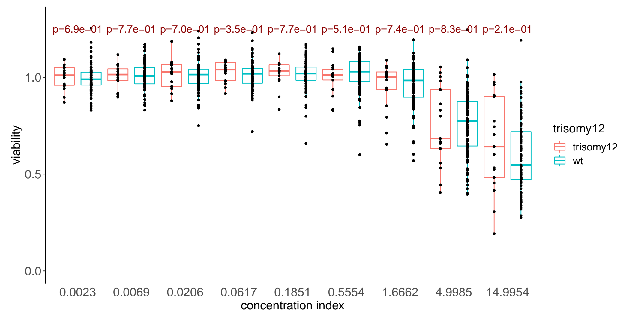
PD407824
