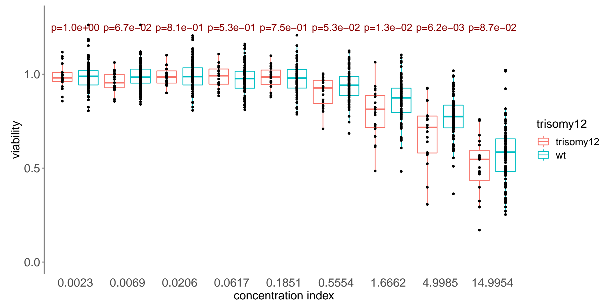
CGI1746
