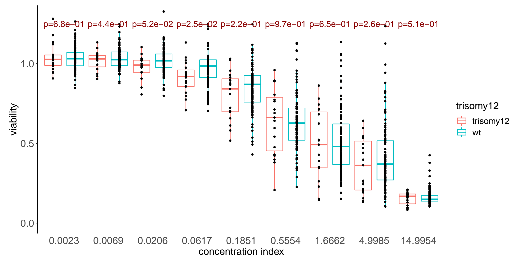
AT9283
