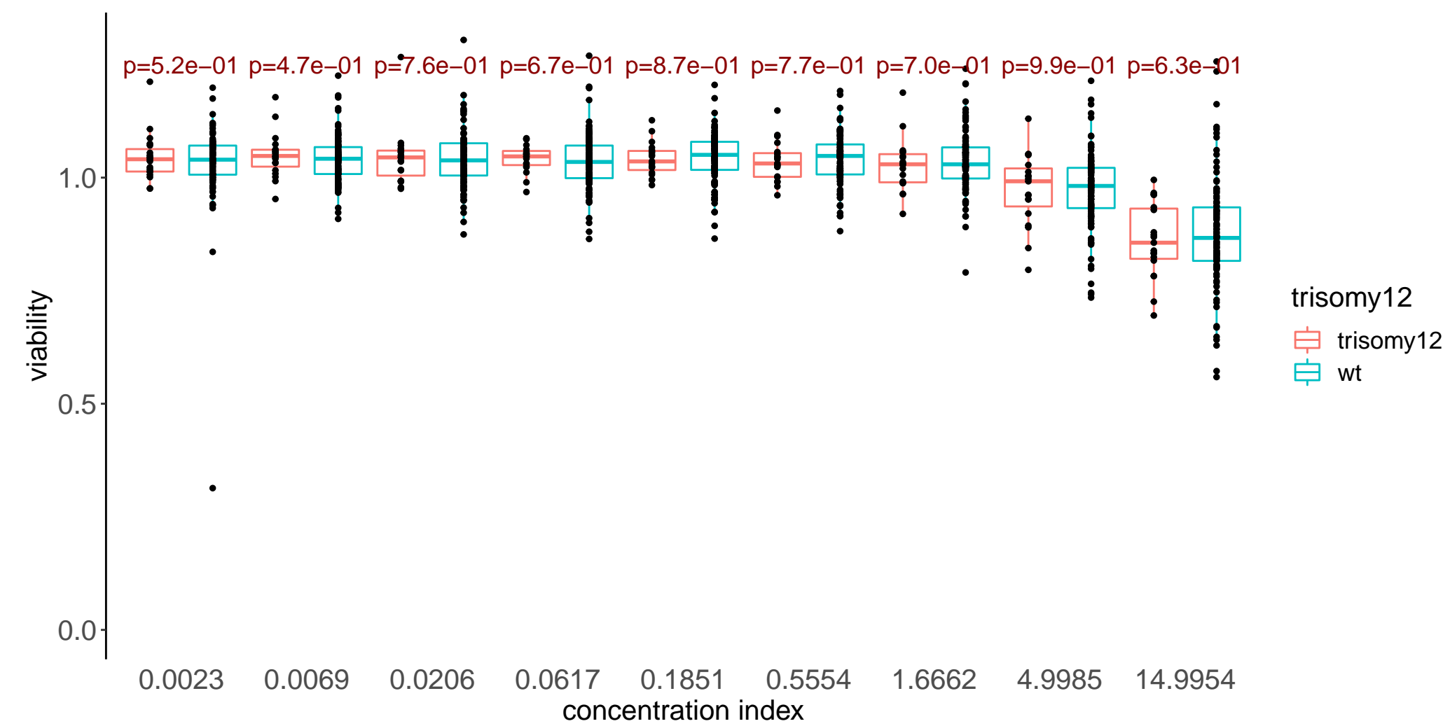
NSC-87877
