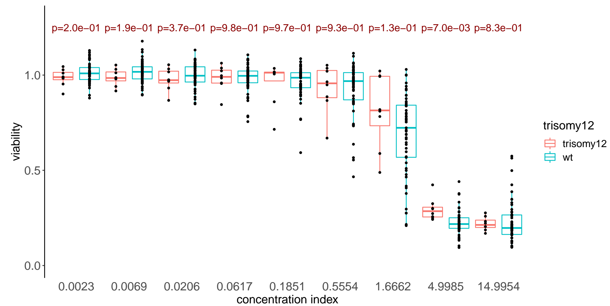
SD50.1
