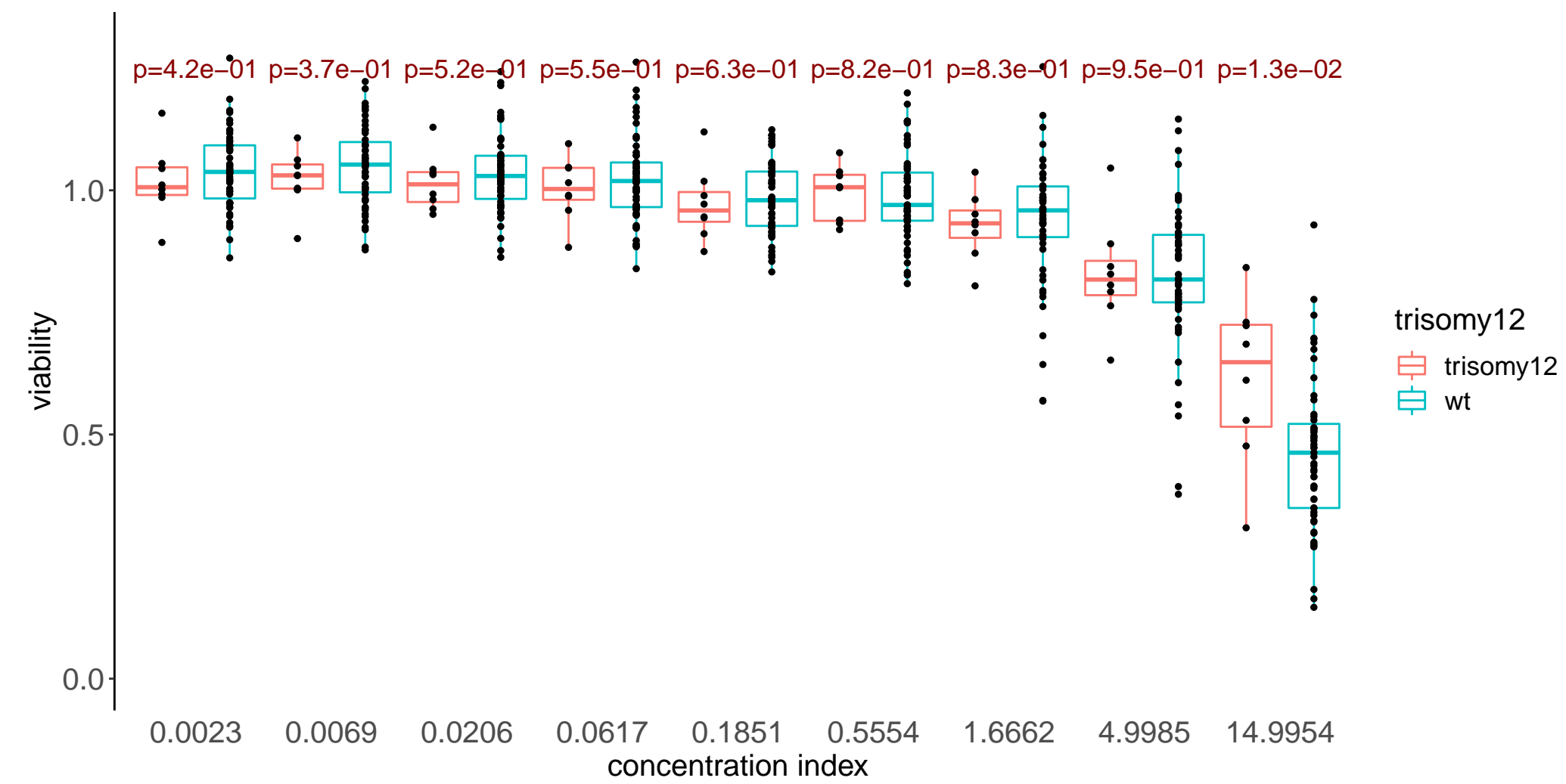
SB225002
