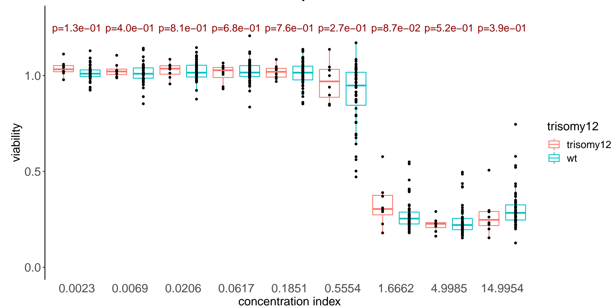
Thiostrepton
