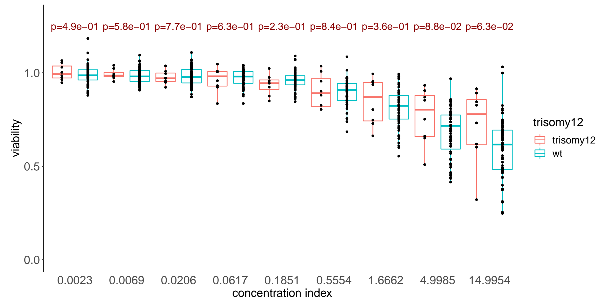
Midostaurin
