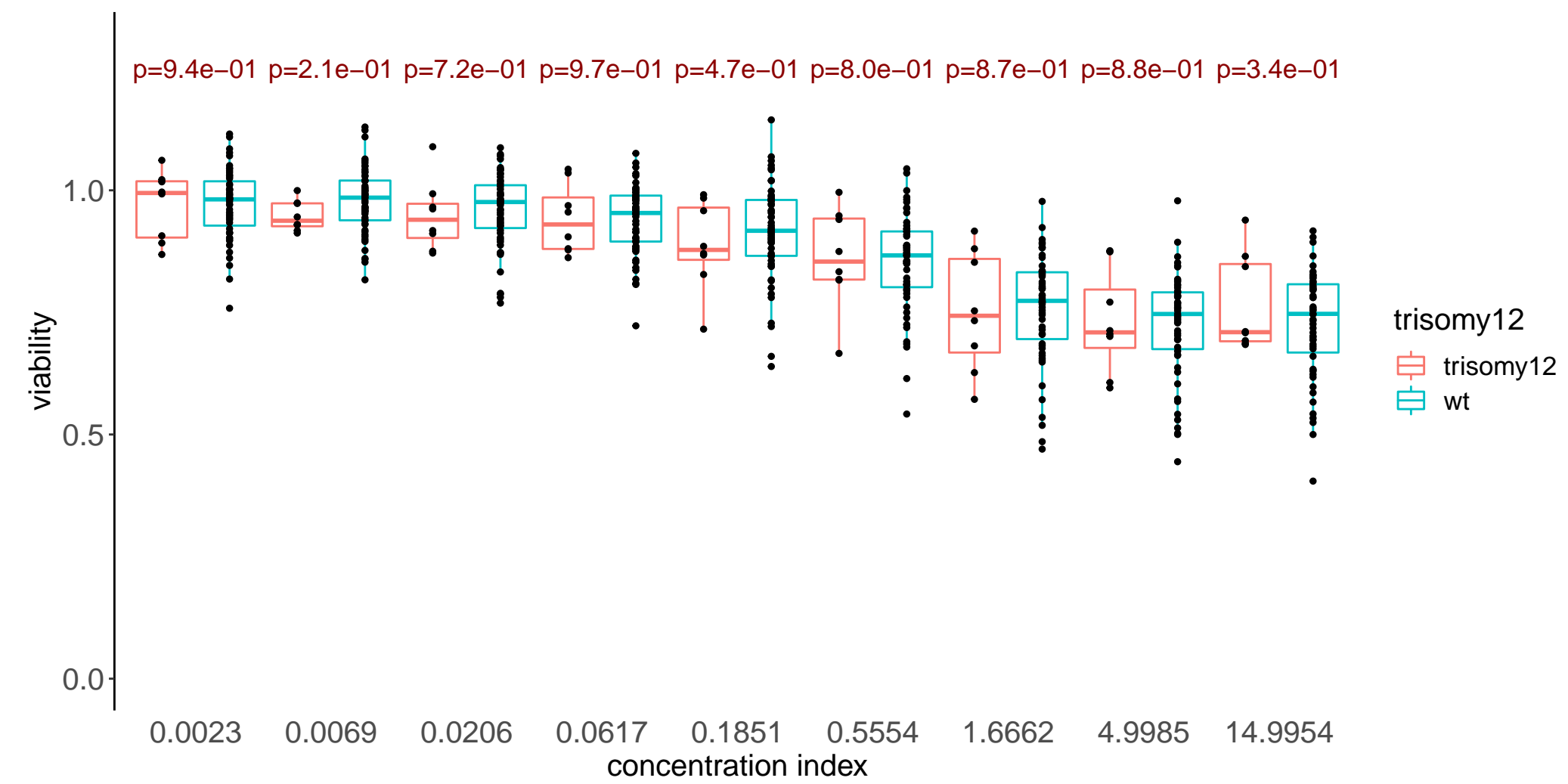
Pentostatin
