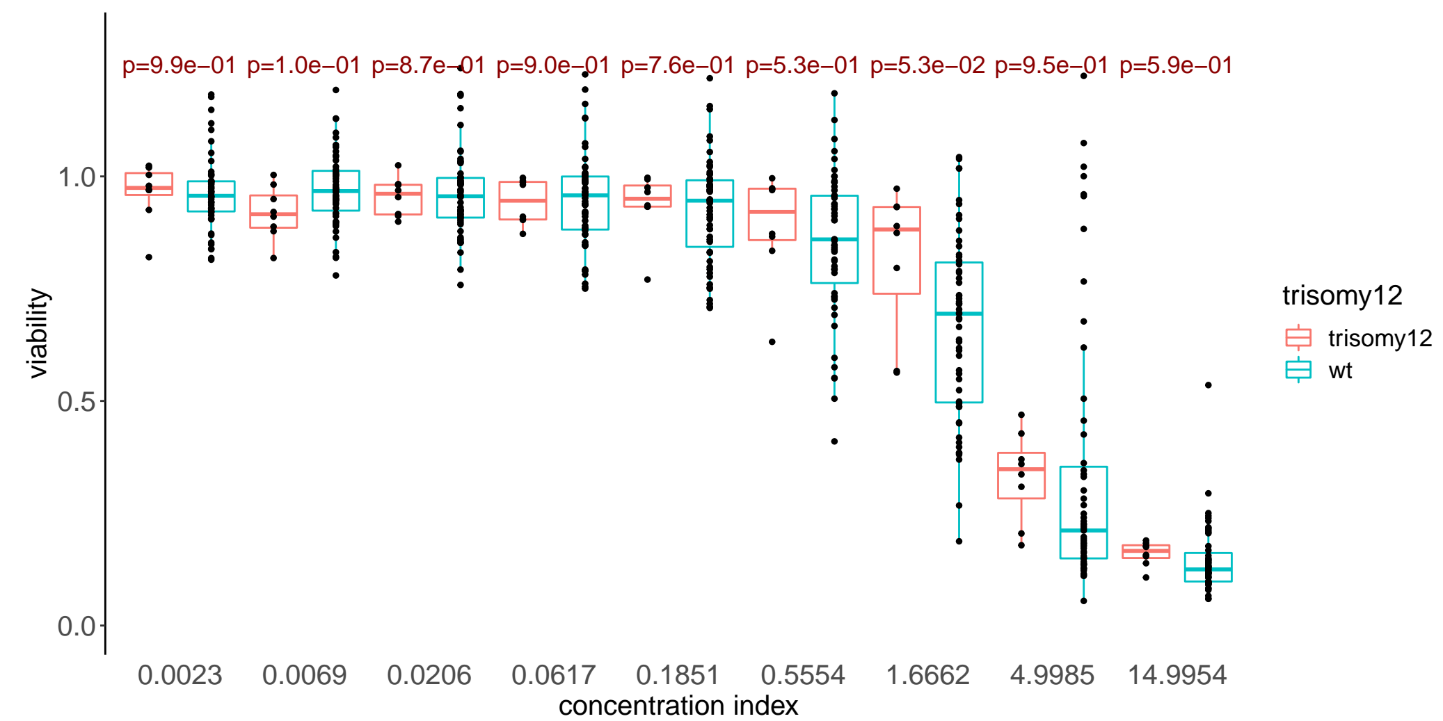
MIS43.1
