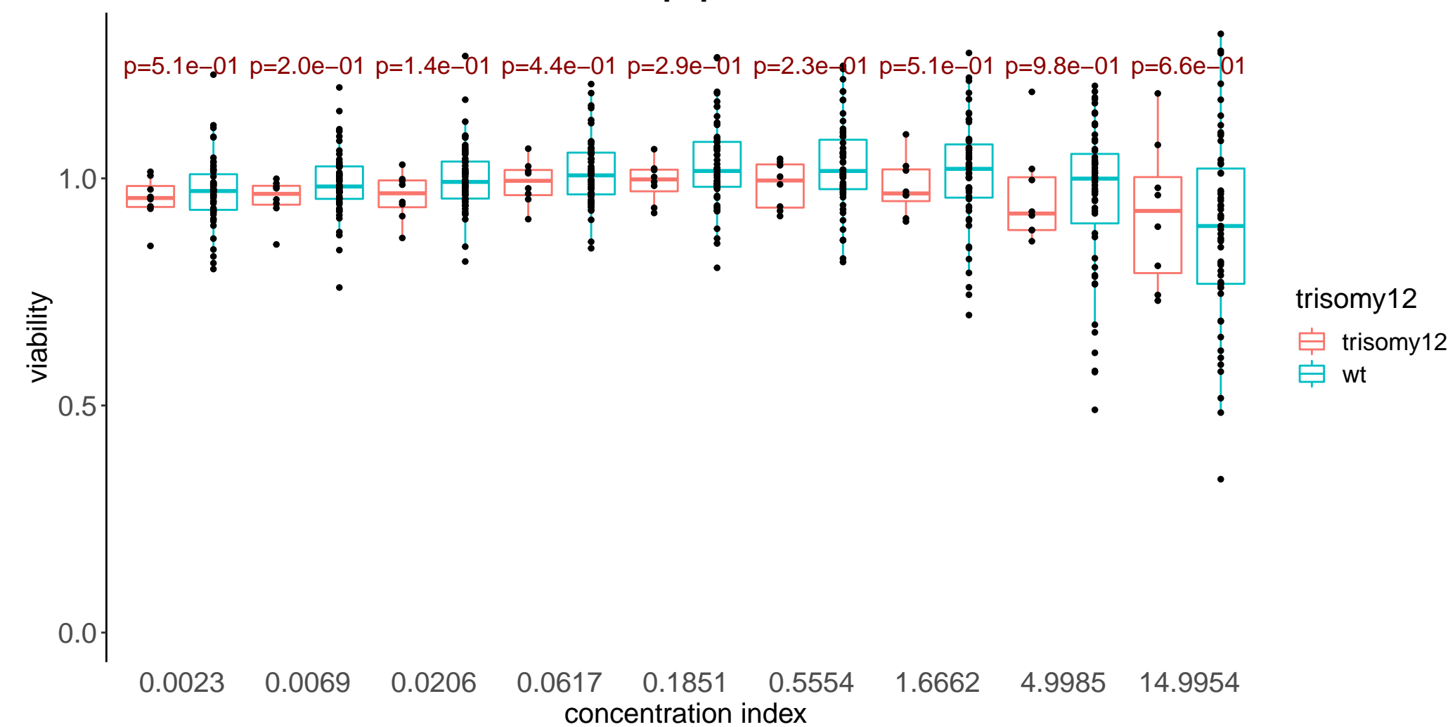
Calpeptin
