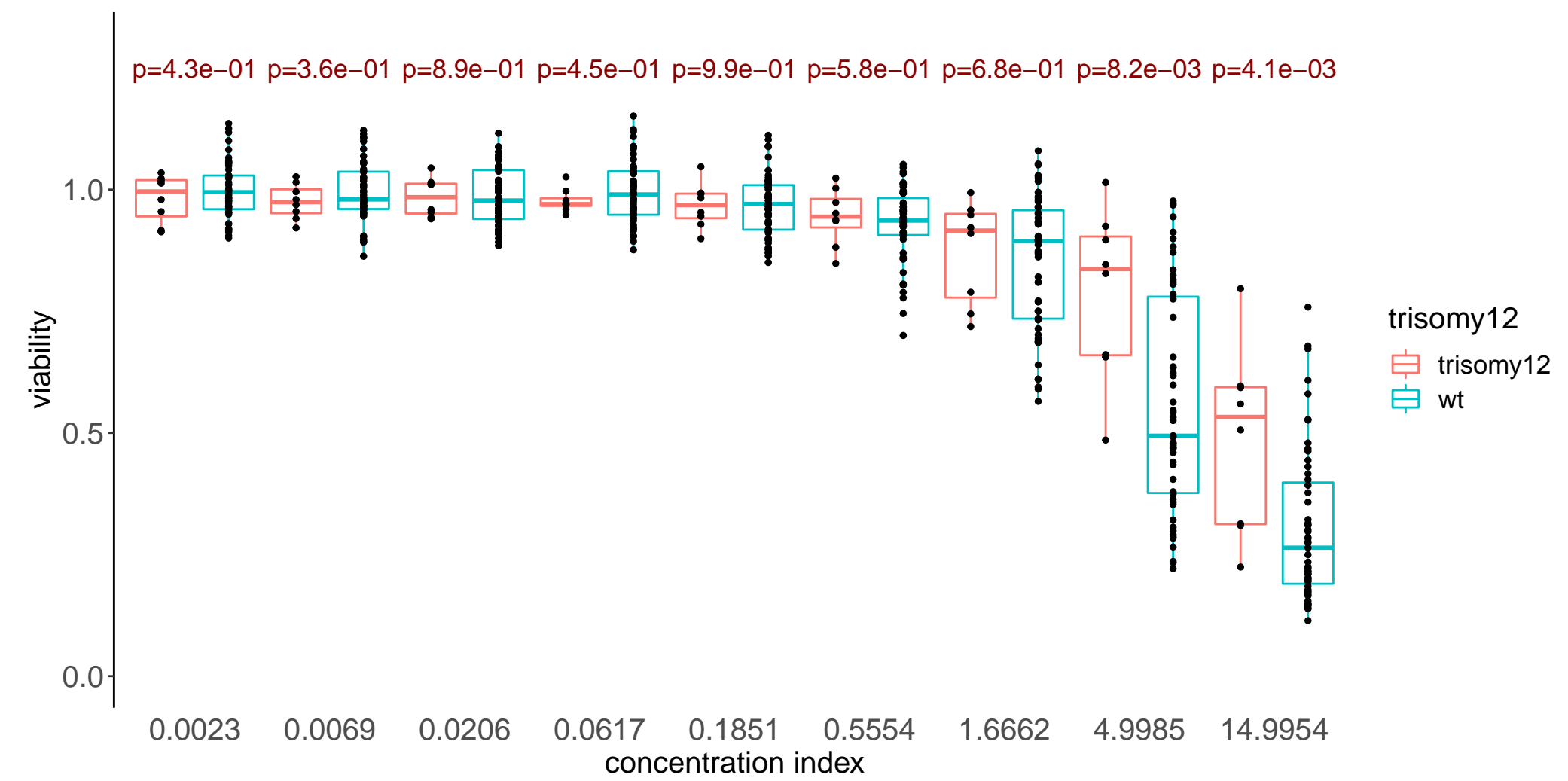
NSC-74859
