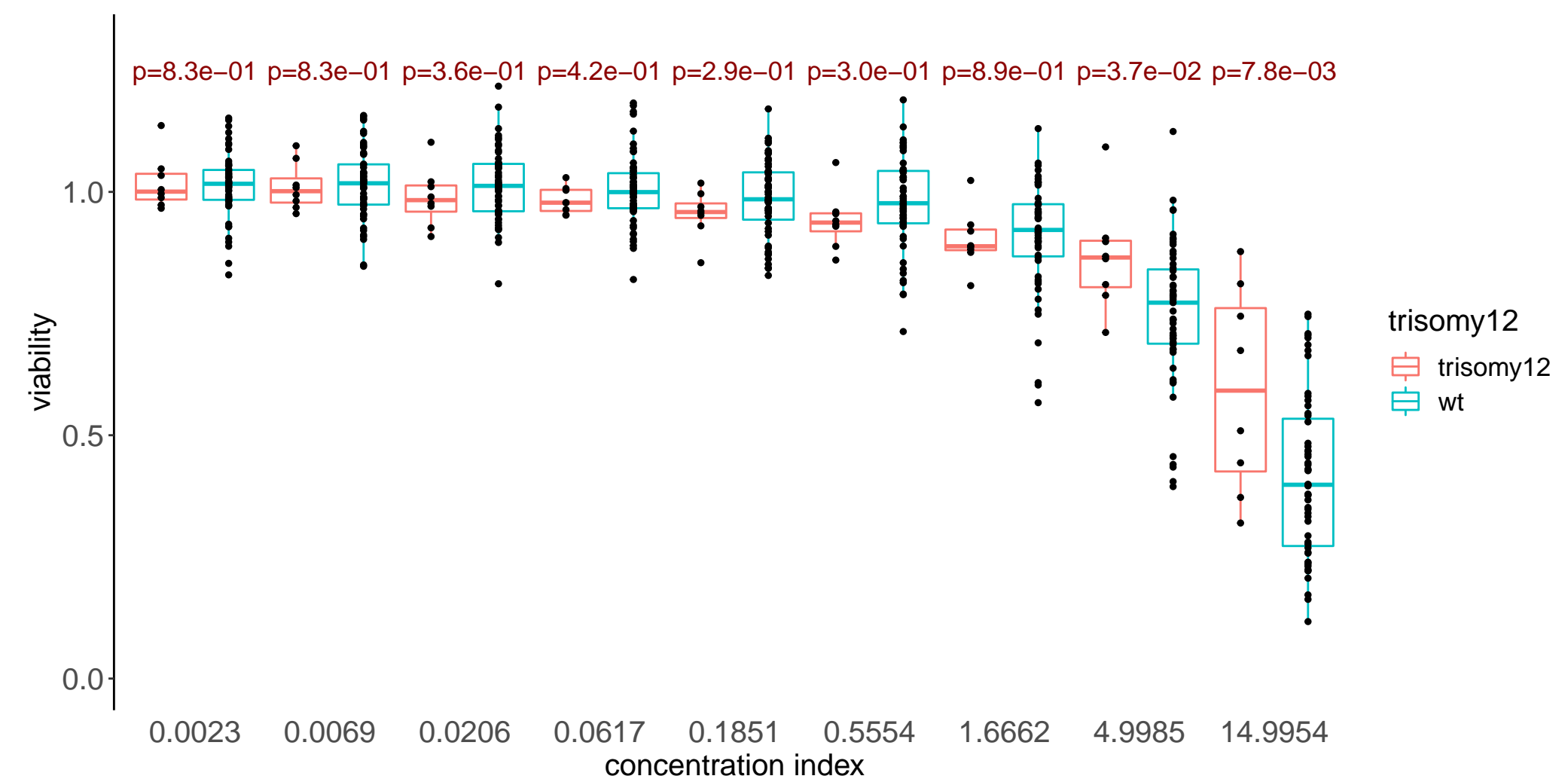
LB42708
