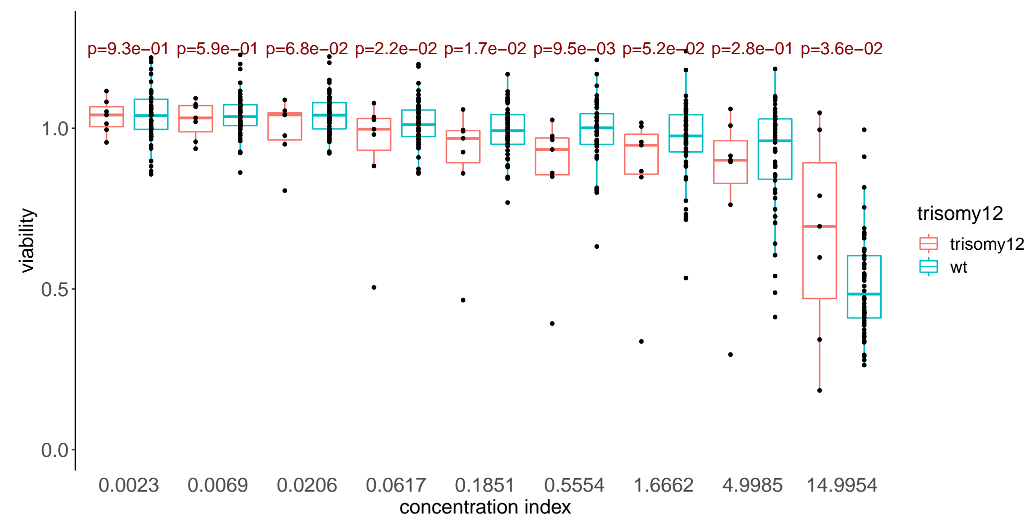
PRT062607
