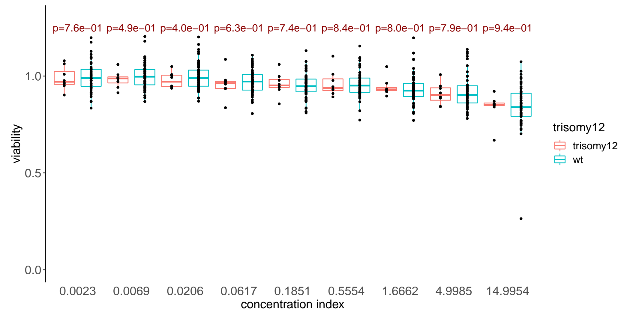
TCS PIM-1 1
