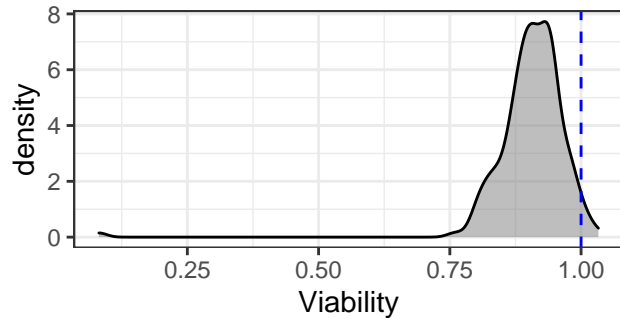
Sabutoclax
