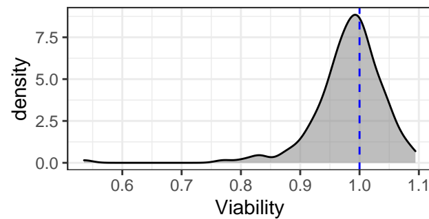
FTI-277 TRIFLUOROACETATE
