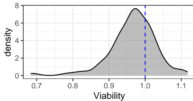
Pictilisib
