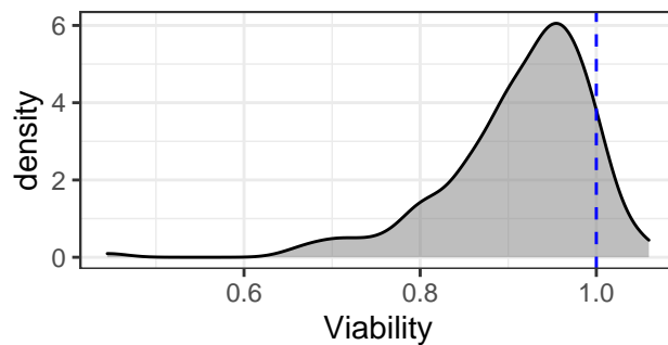
Actinonin
