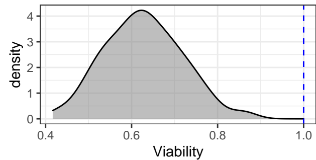
MK-2206
