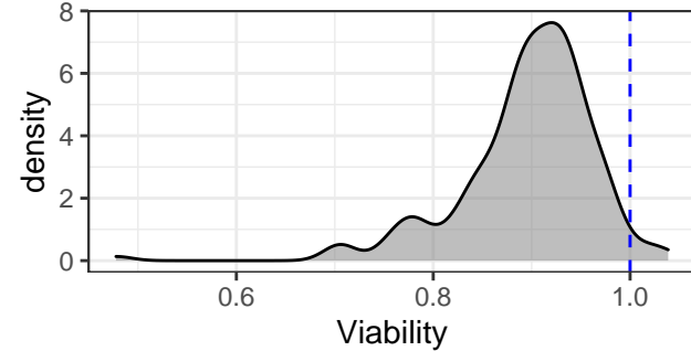
PAZOPANIB
