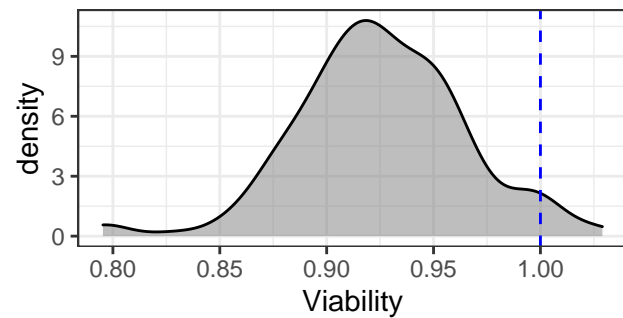
Foretinib
