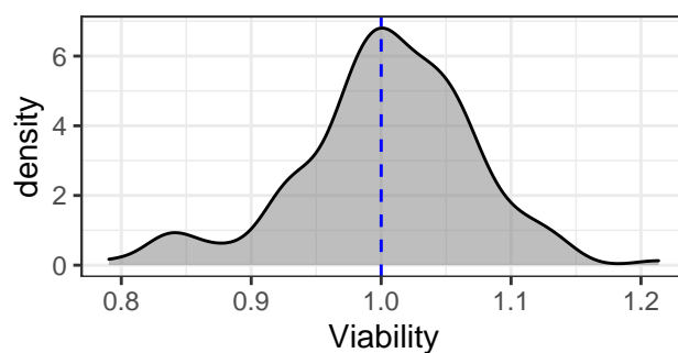
Venetoclax
