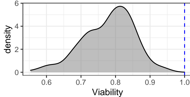
Actinonin
