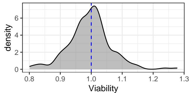
Acadesine
