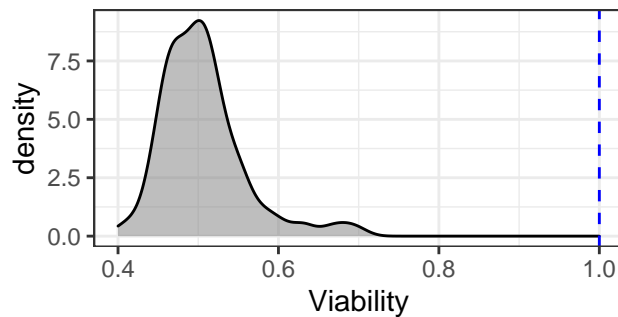
Doramapimod
