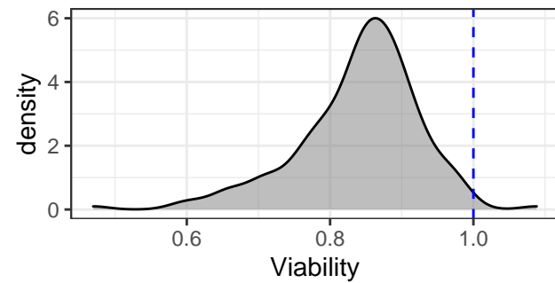
SD50.1
