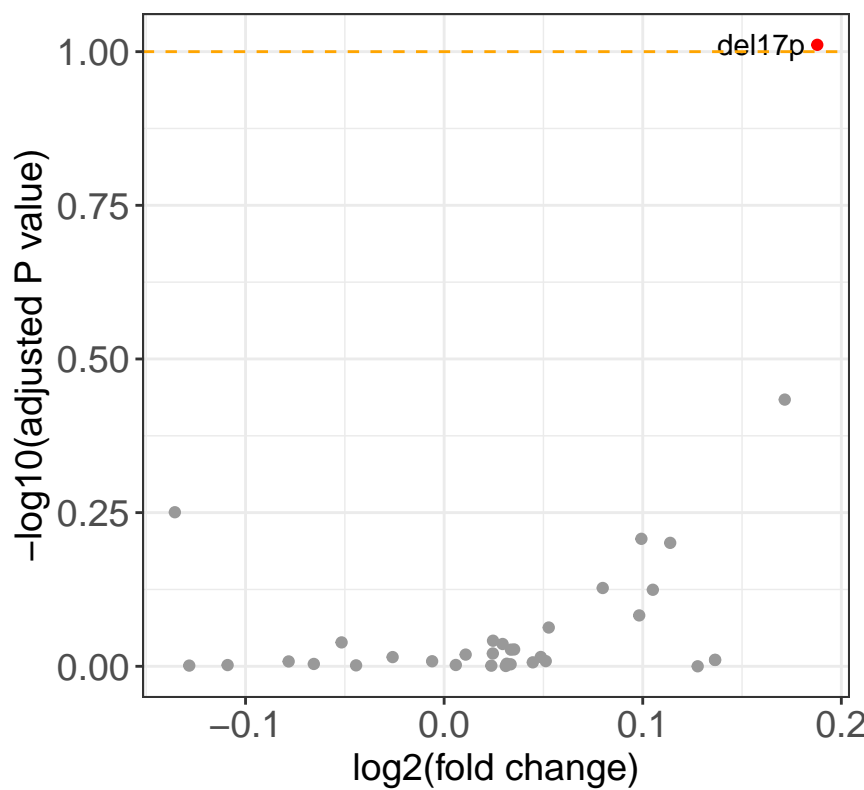
Luminespib
