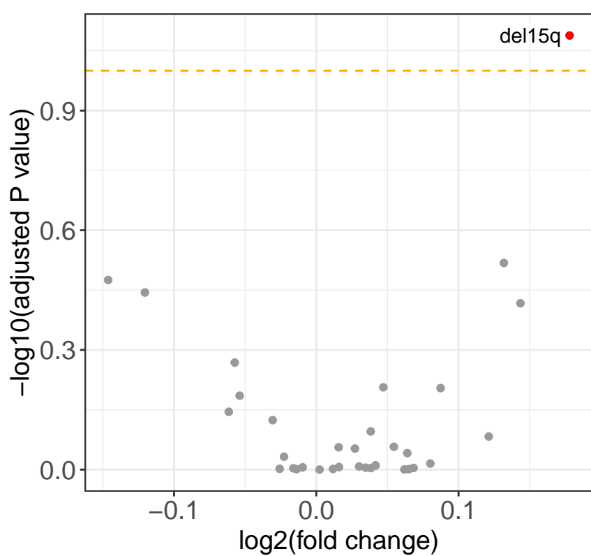
RN486
