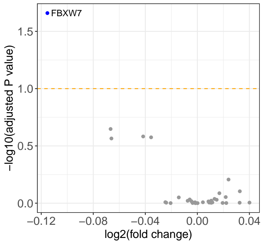
GSK650394
