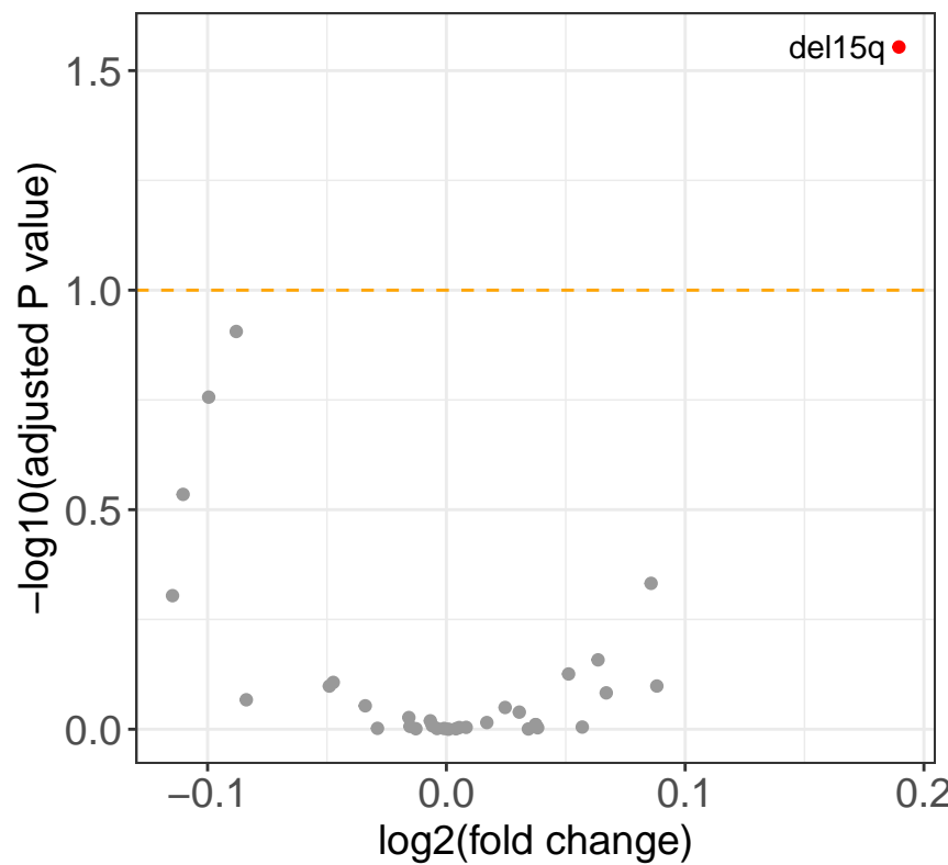
Calpeptin
