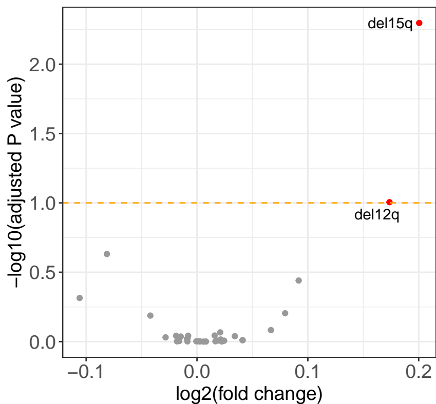
GSK2606414
