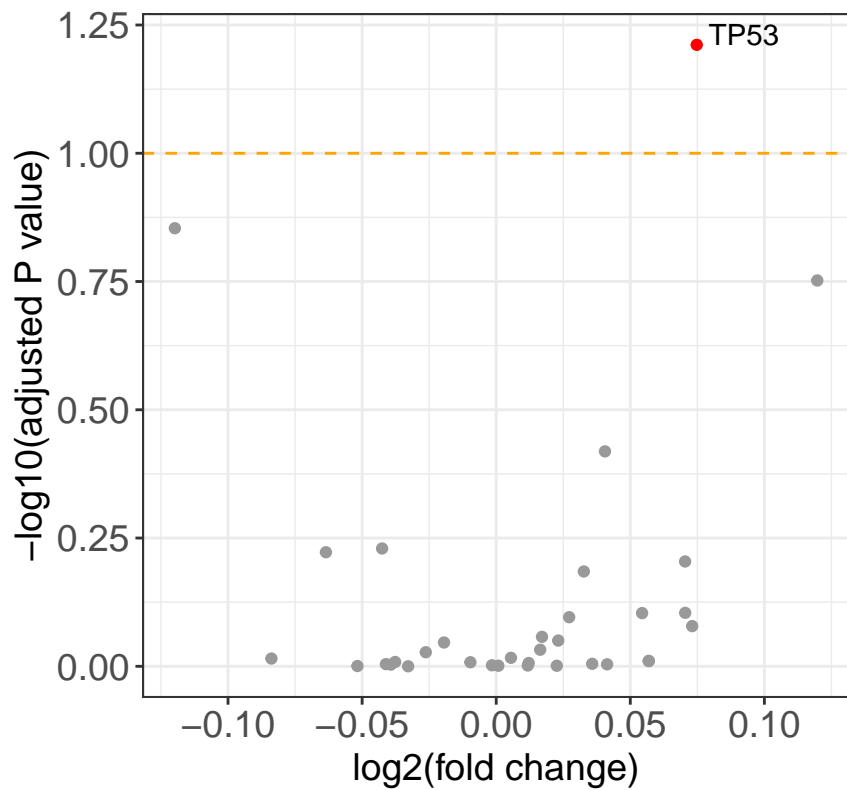
Nutlin-3a
