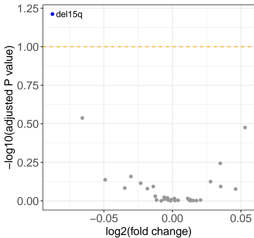
UMI-77
